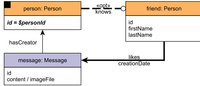
Figure B.2: Pattern of LDBC SNB Interactive Complex Read 7
