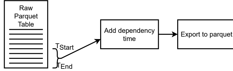
Figure 3.4: Creation of the update streams. The rows from the Parquet file from the time split T_{Start} are extracted and afterward the dependency time is added depending on the entity. The result is exported to Parquet.
