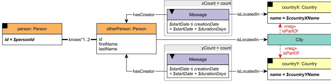
Figure 3.7: Pattern of LDBC SNB Interactive Complex Read 3
