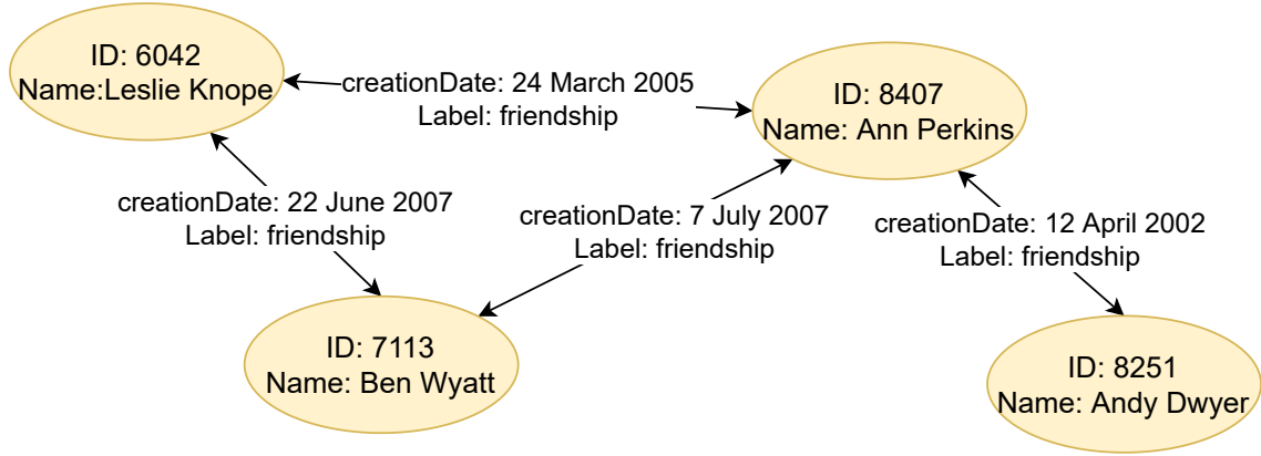
Figure 2.1: Example of a property graph. Yellow ellipses show the Person nodes with the properties ID and Name, connected by relationships with the creation date of the friendship as property.
