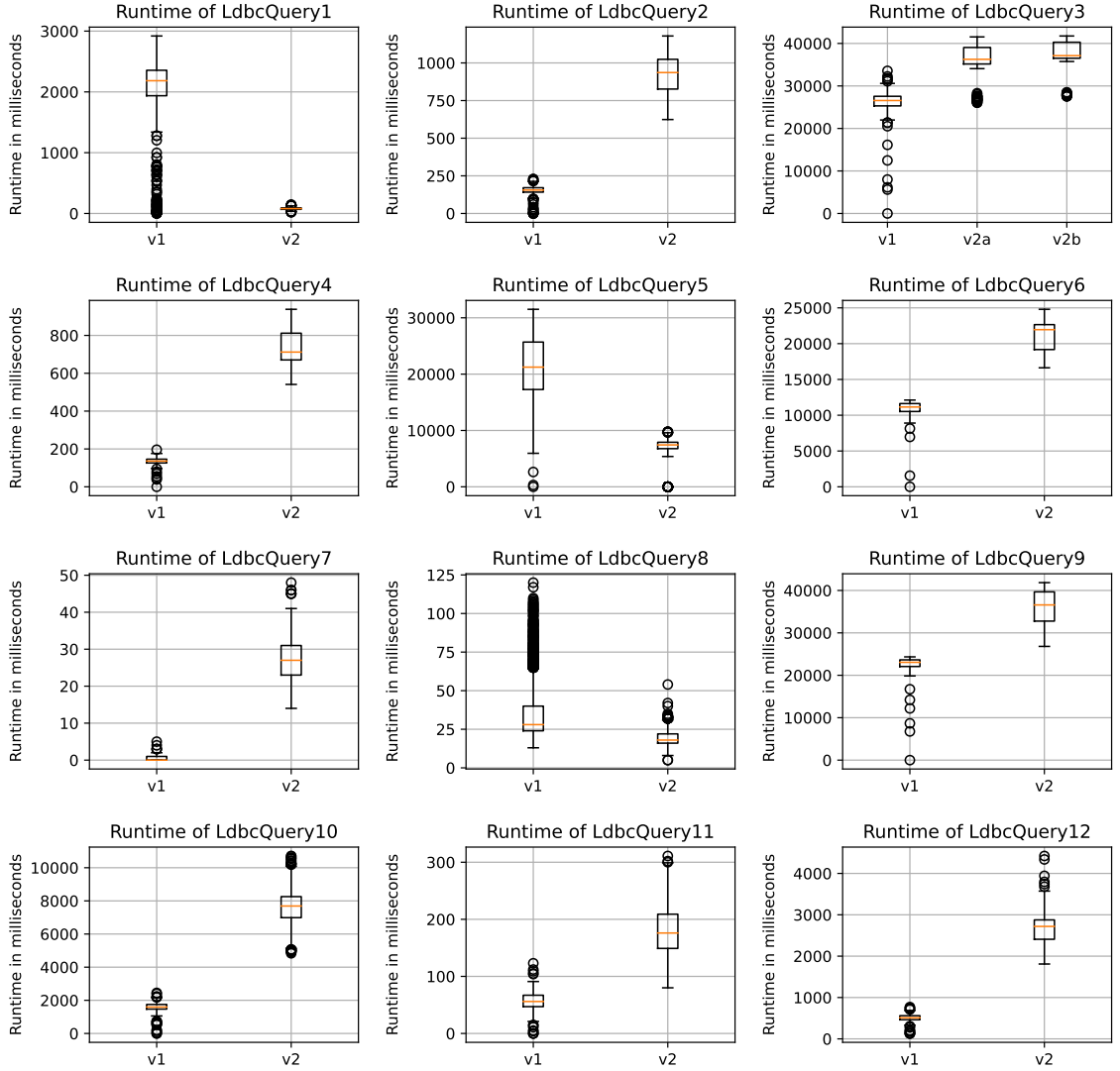
Figure 4.4: Parameter Curation: Curated v1.0 vs. curated v2.0 using Neo4j with SF30. For query3, v2a and v2b denote the variants of the query.
