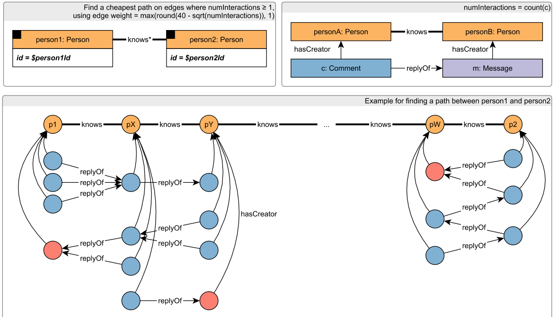
Figure 3.11: Pattern of the new LDBC SNB Interactive Complex Read 14
