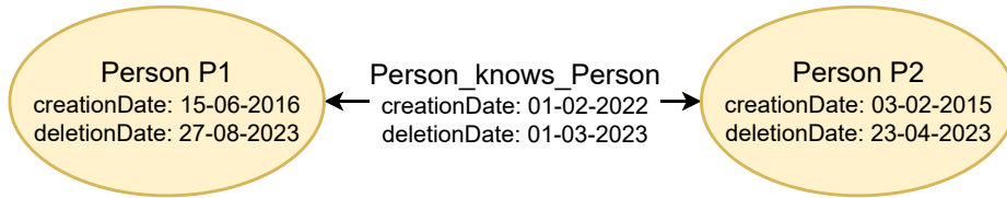
Figure 3.2: Example of lifespan management of an entity and edges. Each node and vertex has a creationDate and deletionDate specified.
