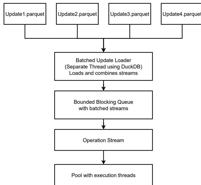
Figure 3.14: Batched loading of the update streams using DuckDB
