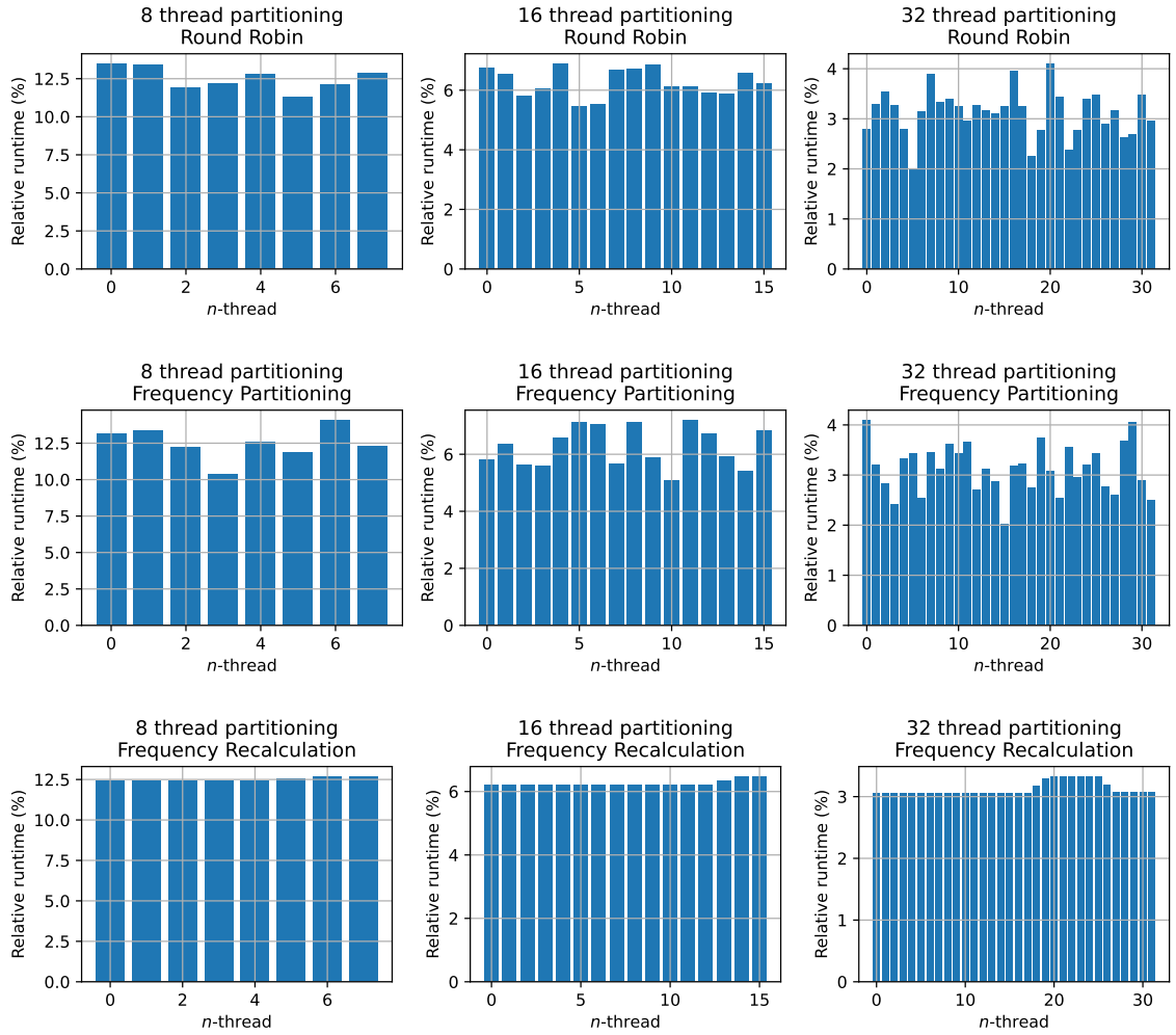
Figure 8.1: Workload distribution: relative runtimes per thread for three different partitioning strategies.
