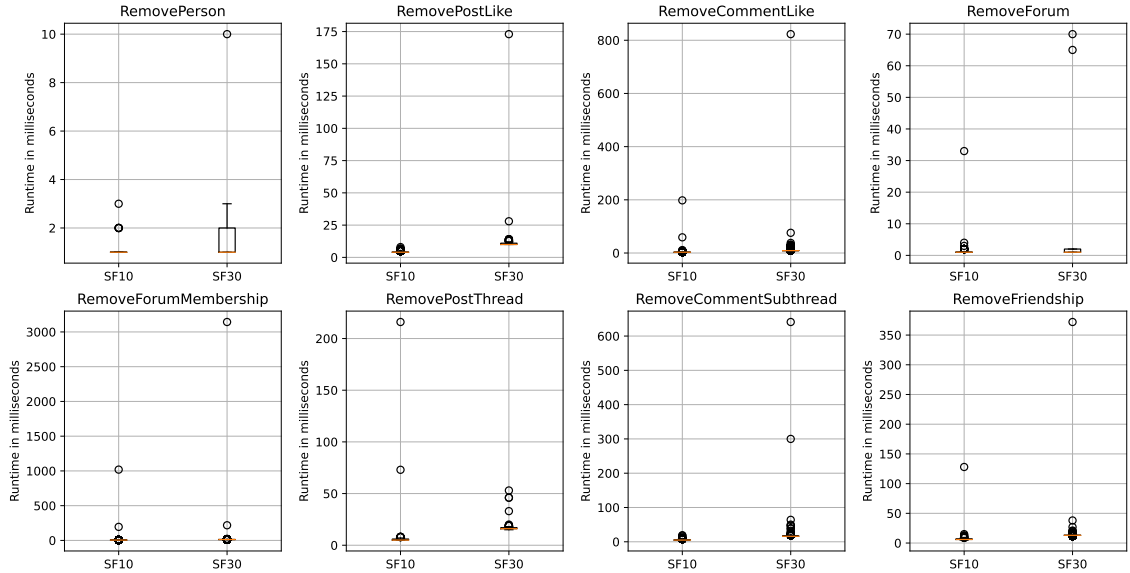
Figure 4.9: Effect of deletes: Runtimes of delete queries using Umbra for scale factors SF10 and SF30.
