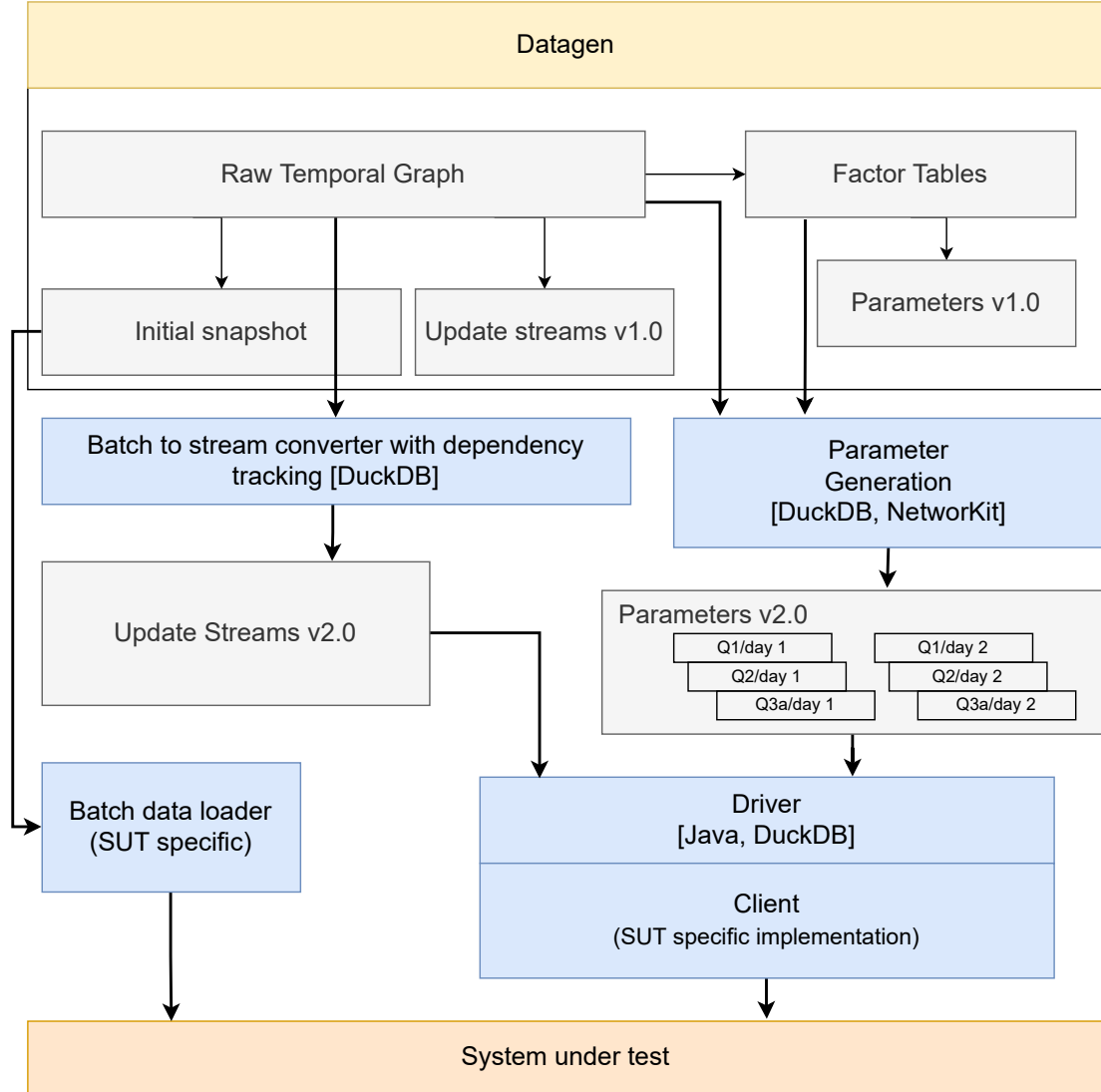
Figure 3.1: Schematic overview of key changes in the Interactive benchmark. The changes are colored blue . The data artifacts are colored grey . Components part of LDBC SNB but not changed in this thesis are marked yellow . Components not part of LDBC SNB are marked orange .
