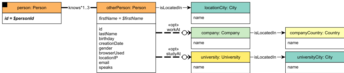
Figure 3.5: Pattern of LDBC SNB Interactive Complex Read 1
