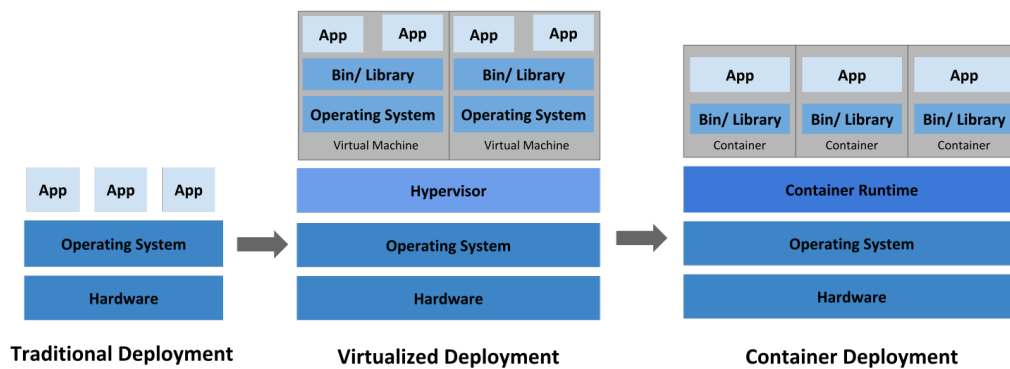
Figure 6.1: Mapping from virtual machine with applications to Kubernetes. Image from (6)
