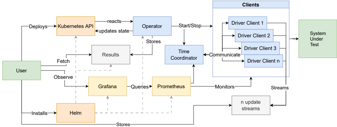
Figure 7.2: Distributed driver architecture. Orange shows the elements that are present in the Kubernetes cluster, Yellow are the external components that need configuration, Blue are the components specifically for the distributed driver.
