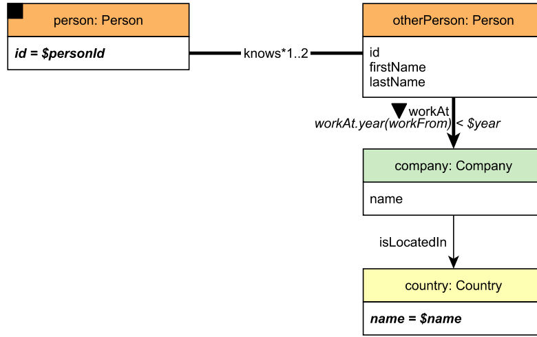
Figure B.6: Pattern of LDBC SNB Interactive Complex Read 11
