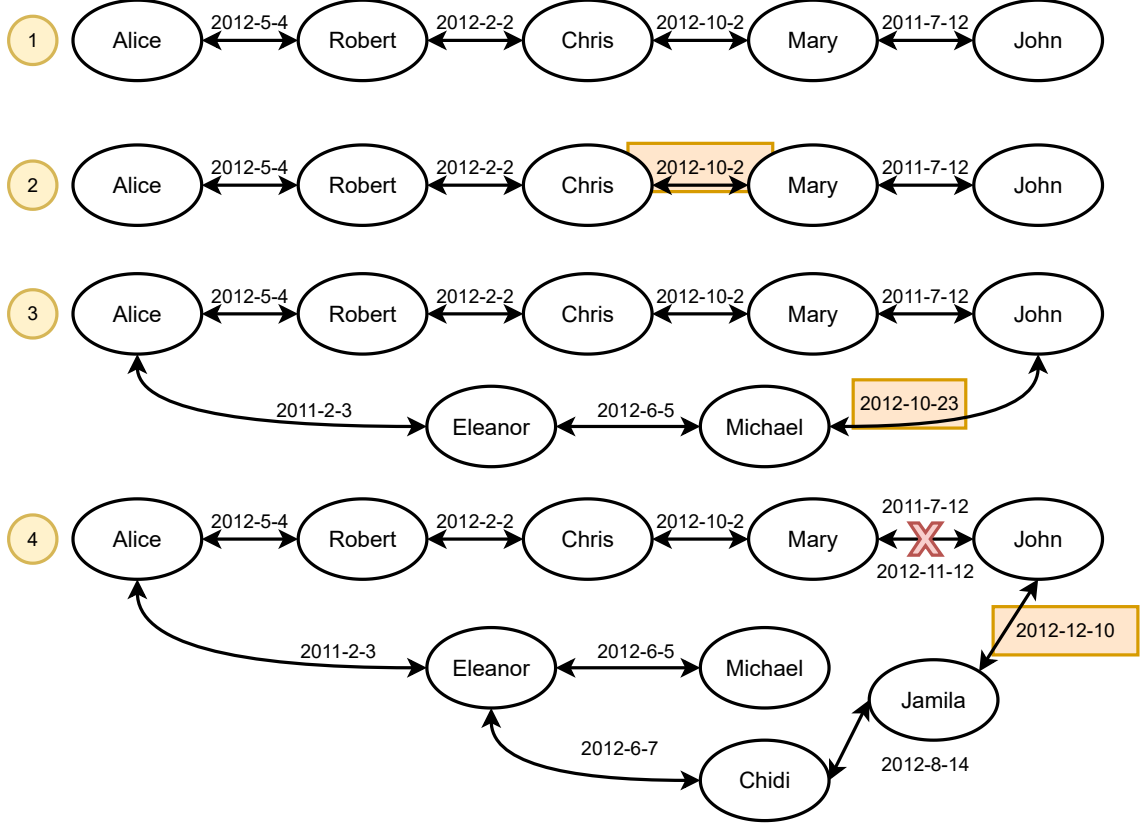
Figure 3.13: Example of the problem of temporary paths in the Spark Data set.
