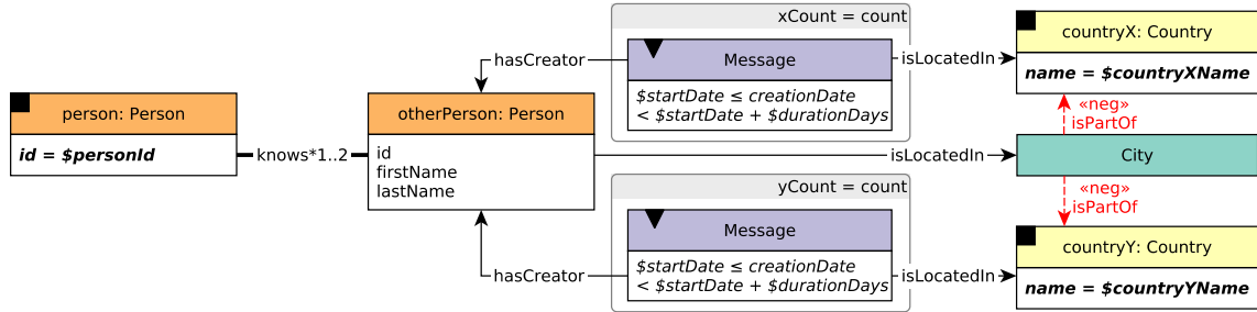
Figure 2.7: Query template Query 3 (1). The dashed red lines note negative conditions, i.e., these edges must not exist in the graph.
