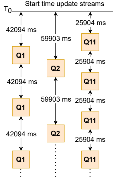
Figure 2.8: Example of scheduling of complex read queries with an update interleave of 1619 ms and frequencies Query1=26, Query2=37 and Query11=16, see Equation 2.2
