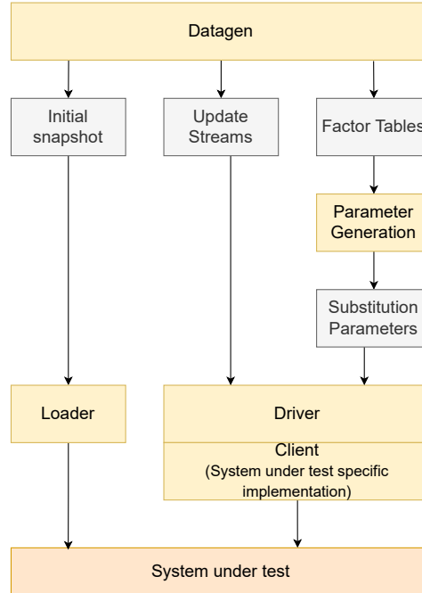
Figure 2.4: Overview of the software components and data artifacts of the Interactive workload. Legend: Yellow are the software components, grey the data artifacts and orange the DBMS tested.
