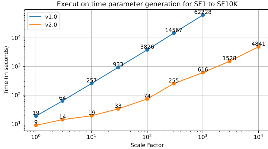
Figure 4.3: Runtime of the parameter generators for Interactive v1.0 and v2.0. The labels show the runtime in seconds.
