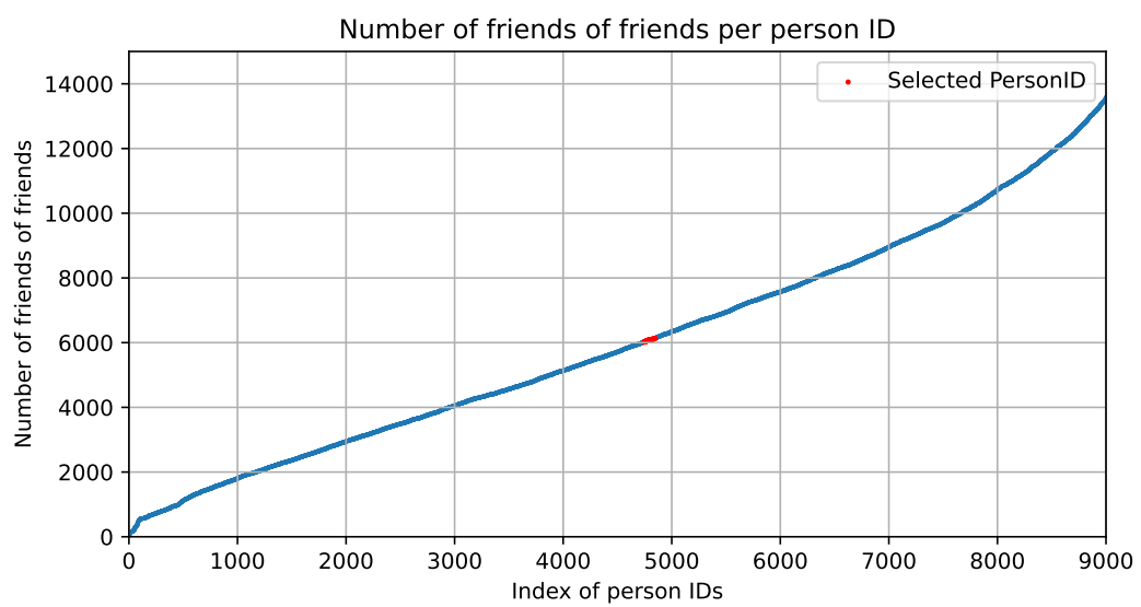
Figure C.3: Selected window of person IDs in the distribution of number of friends of friends
