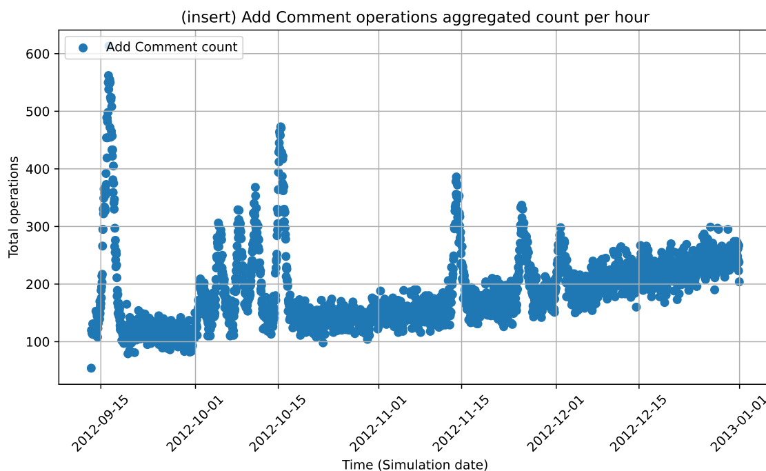
Figure 2.3: Example of a spiking event in the Hadoop Datagen update streams (comment inserts) for Scale Factor 1. Update operations are bucketized per hour according to their simulation timestamp.
