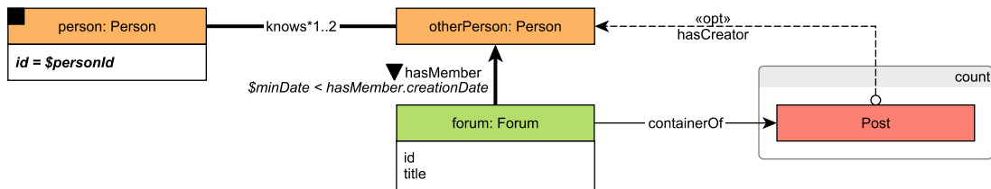
Figure 3.9: Pattern of LDBC SNB Interactive Complex Read 5
