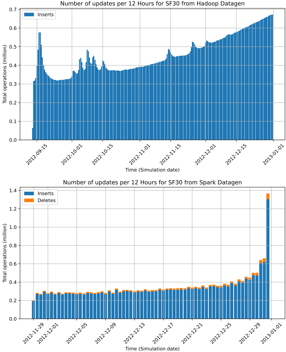
Figure 4.1: Number of events per 12 hours for Hadoop and Spark during the simulation time of the benchmark.
