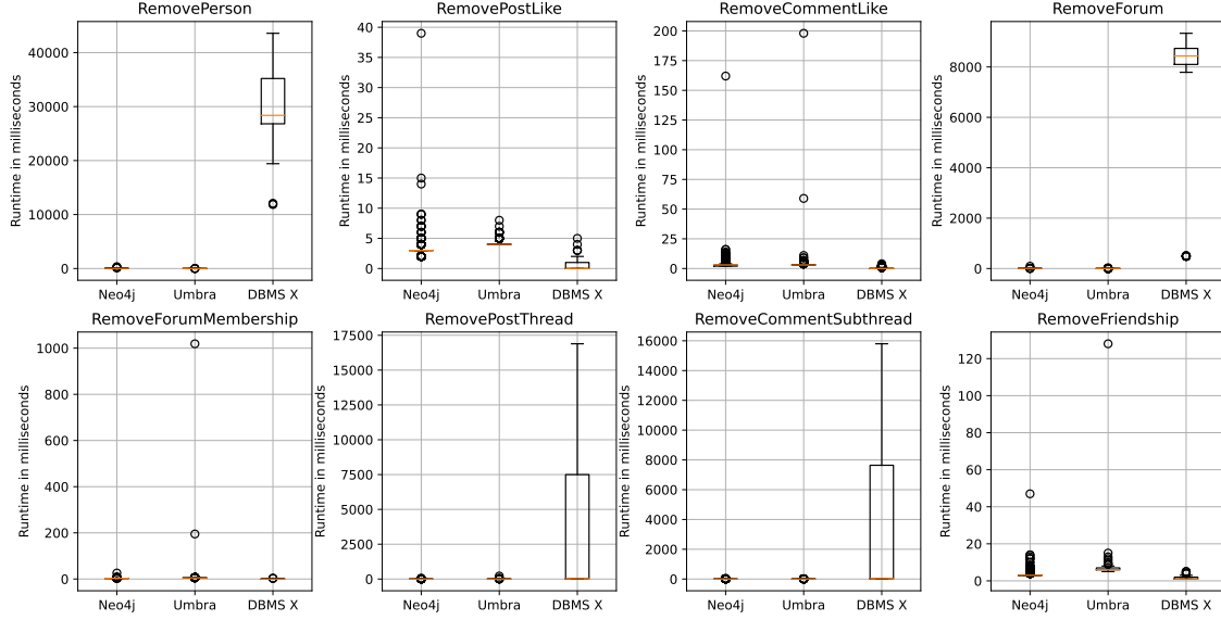
Figure 4.10: Effect of deletes: Runtime comparison of delete queries for Neo4j v4.4.1, Umbra and DBMS X using SF10 and 750,000 update operations.
