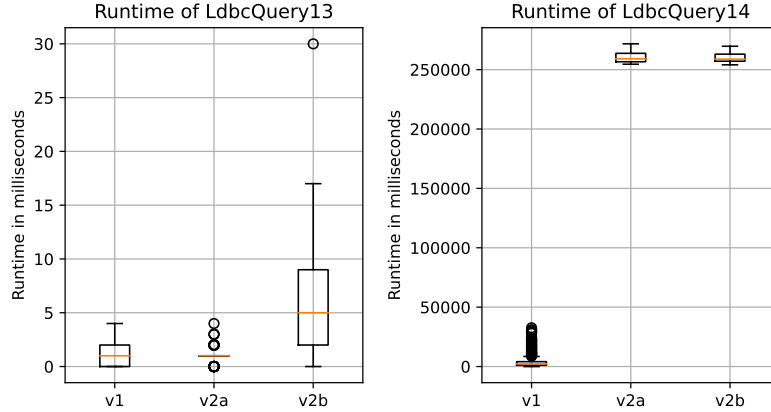
Figure 4.7: Path queries: Runtimes for path queries with interactive v1.0 and interactive v2.0 using Neo4j. Note that Q14 is changed between v1.0 and v2.0, with v2.0 performing the computationally much more difficult cheapest path problem.
