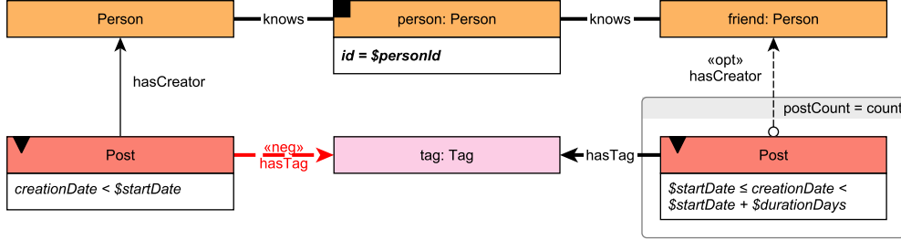
Figure 3.8: Pattern of LDBC SNB Interactive Complex Read 4
