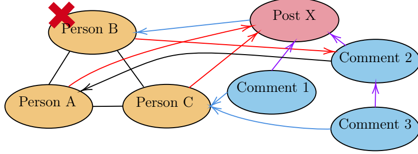
Figure 1.1: Example of a deletion in the SNB graph. The red edges are likes from a person to a post/comment, blue edges are creator edges, purple edges are replyOf edges and black edges are knows edges. In case Person B is removed from the graph, the cascading effects cause all nodes and edges to be deleted except Person A, Person C and their knows edge, yielding a deletion of 5 nodes and 12 edges.
