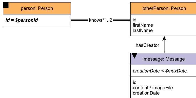
Figure B.4: Pattern of LDBC SNB Interactive Complex Read 9
