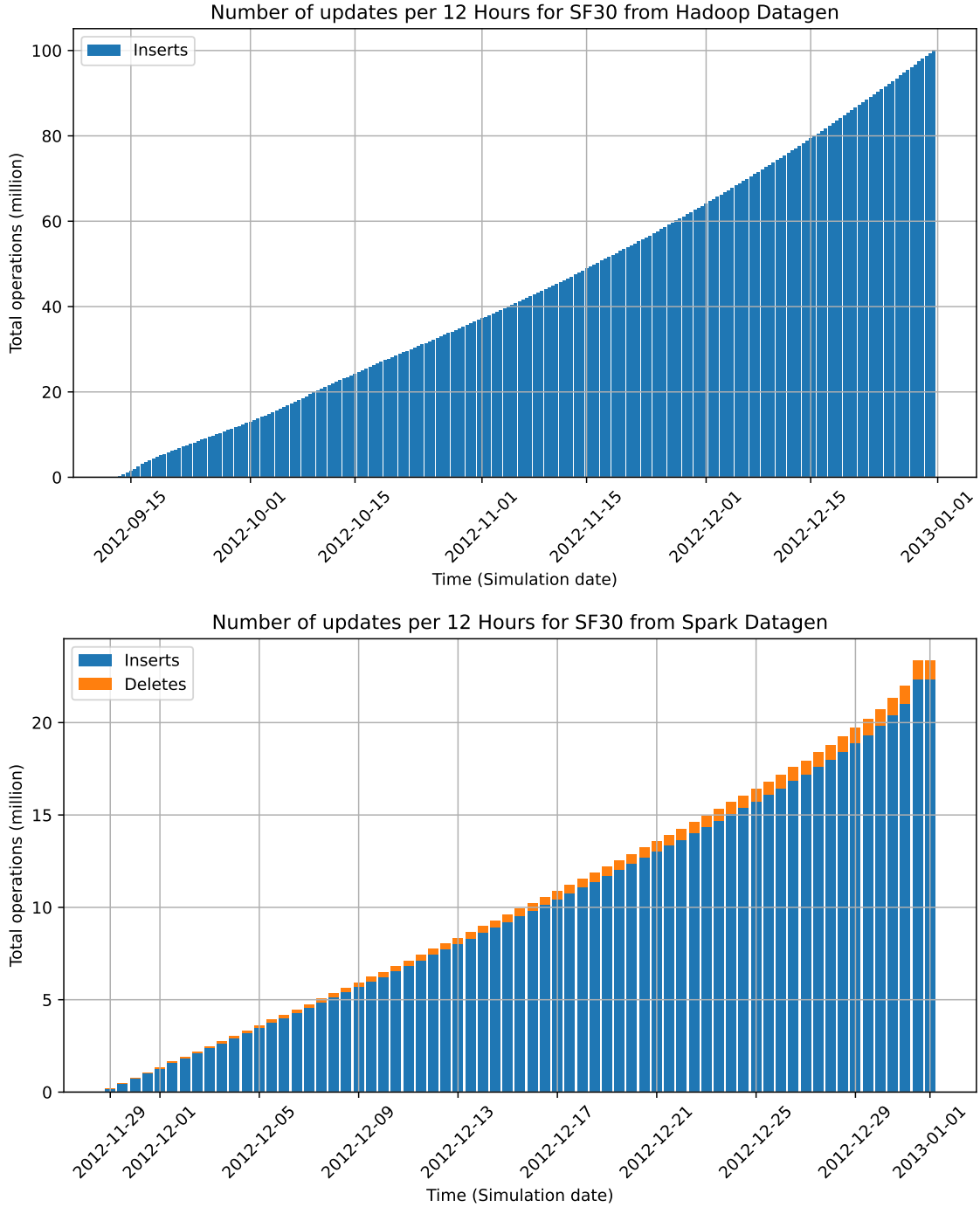
Figure 4.2: Cumulative sum of the number of events per 12 hours for Hadoop and Spark during the simulation time of the benchmark.
