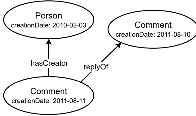
Figure 3.3: Example of an entity with dependencies.
