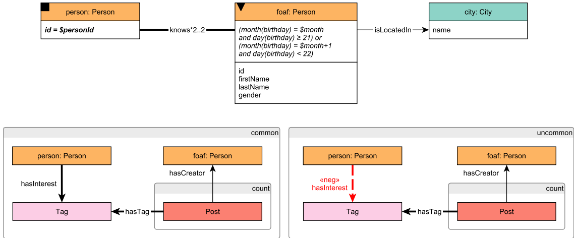
Figure B.5: Pattern of LDBC SNB Interactive Complex Read 10
