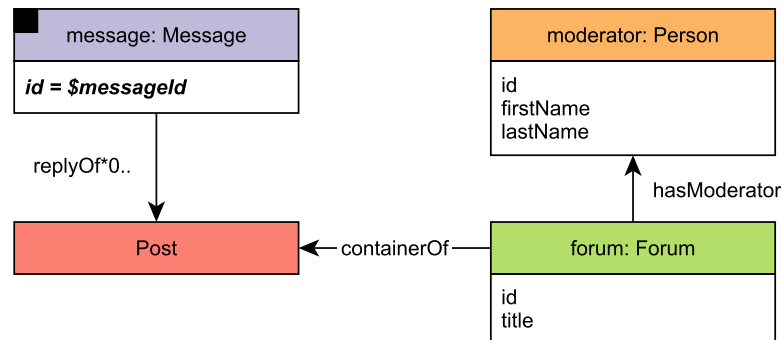
Figure 2.2: Example query: LDBC SNB Interactive short query 6 (1). The input parameter is denoted as $messageId .
