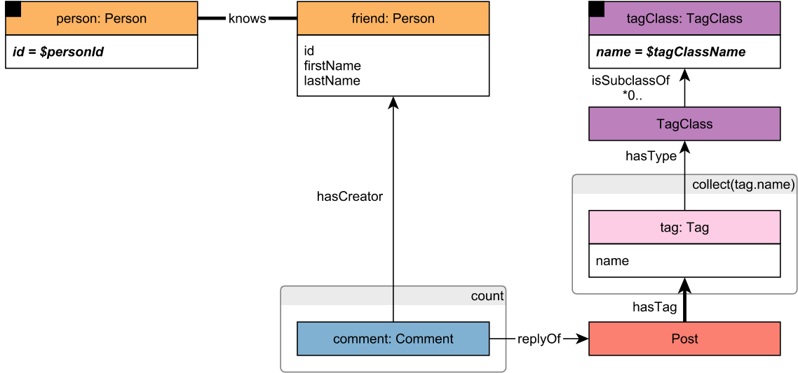
Figure B.7: Pattern of LDBC SNB Interactive Complex Read 12
