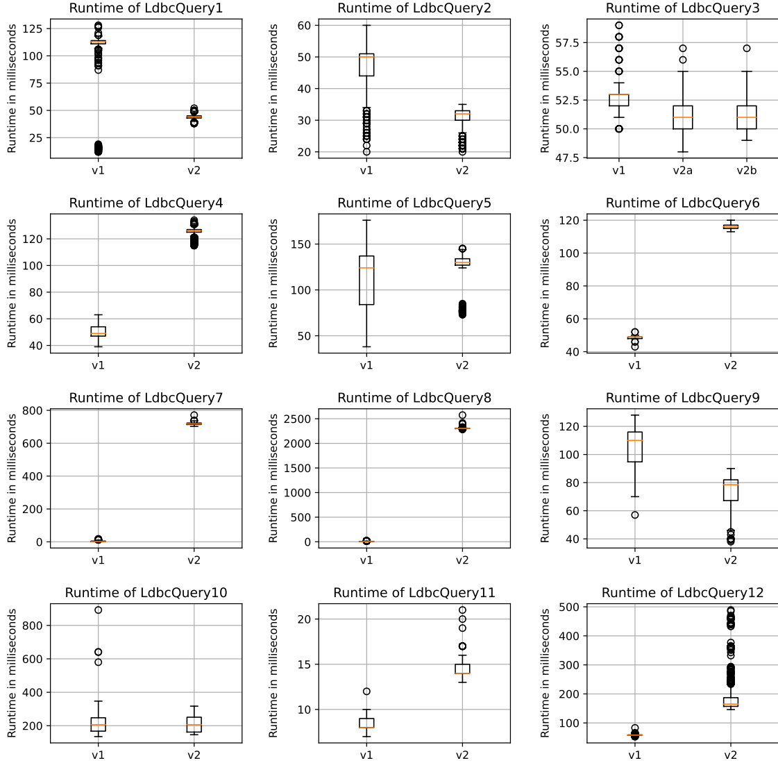
Figure 4.5: Parameter Curation: Curated v1.0 vs. curated v2.0 using Umbra 45f3aae27 with SF30. For query3, v2a and v2b denote the variants of the query.
