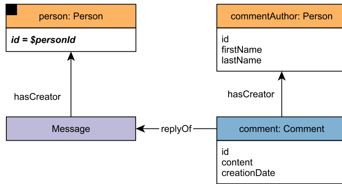
Figure B.3: Pattern of LDBC SNB Interactive Complex Read 8
