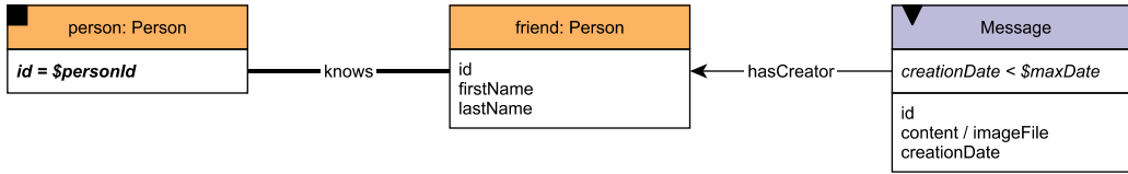
Figure 3.6: Pattern of LDBC SNB Interactive Complex Read 2
