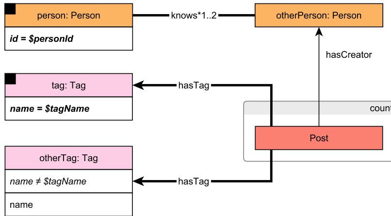
Figure B.1: Pattern of LDBC SNB Interactive Complex Read 6
