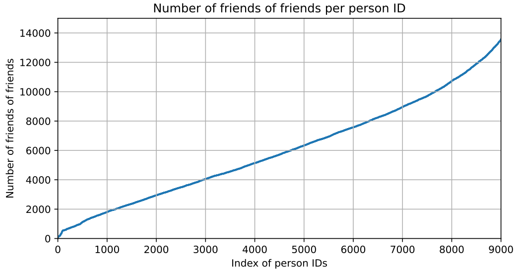
Figure C.1: Distribution of the number of friends of friends per person ID.
