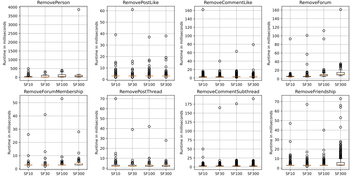
Figure 4.8: Effect of deletes: Runtimes of delete queries using Neo4j 4.4.1 for scale factors SF10, 30, 100 and 300
