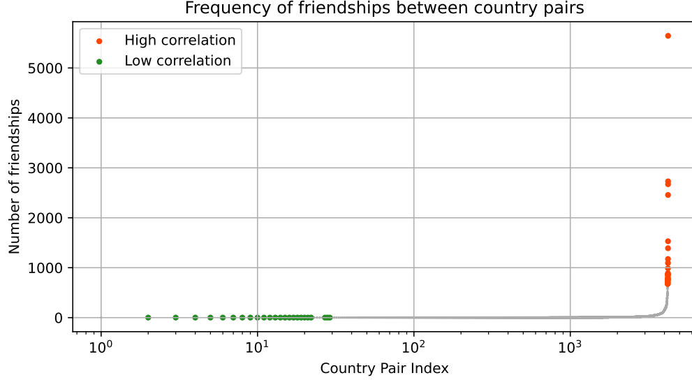
Figure 3.12: Selection of countries in the countryPairsNumFriends factor table on the number of friendships between both countries using the percentile_disc function. Correlated countries (red) are selected using percentile 1.0 and anti-correlated countries (green) are selected using percentile 0.01.
