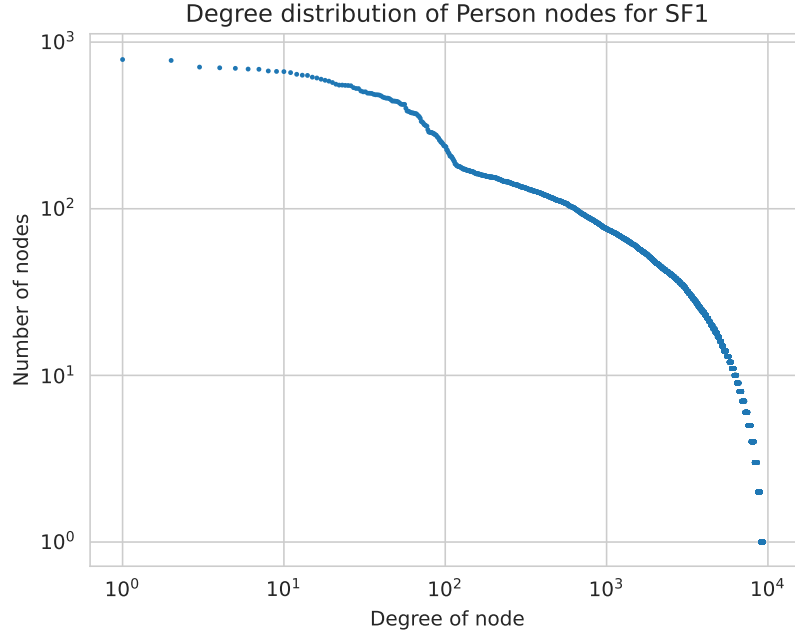
Figure 2.5: Degree distribution of the Person nodes in the SNB graph for Scale Factor 1.
